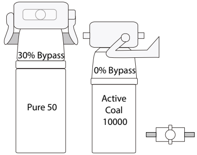
Alternative placement of shutoff valve next to filters. Filters can be mounted in an adjacent cabinet.
